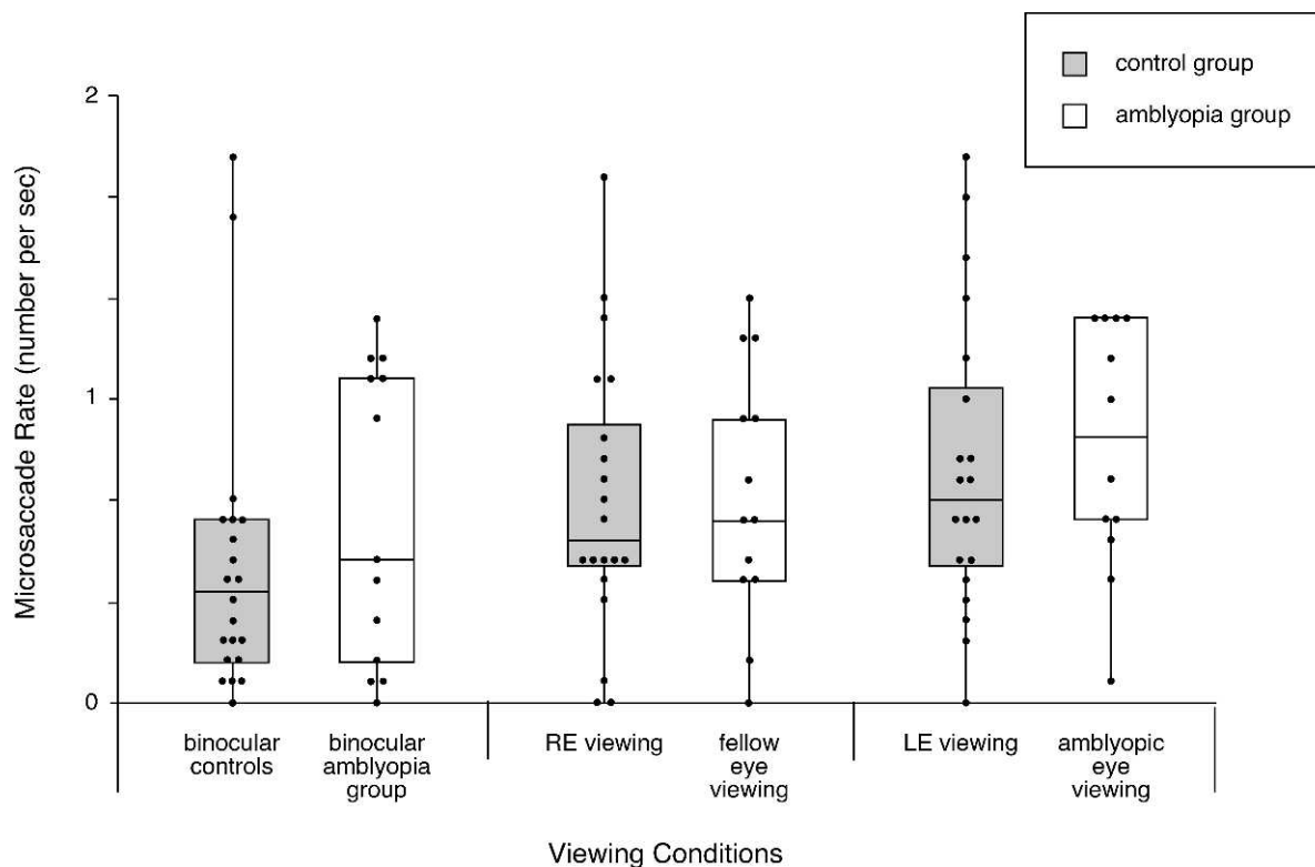
FIGURE 4. Box plots of microsaccade rates for the control and amblyopia groups. Black discs show individual data points shifted horizontally for clarity purposes.
