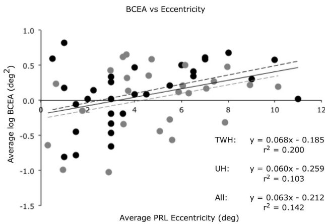
FIGURE 4. Average log BCEA (in log deg 2 ) is plotted against the average estimated PRL eccentricity (in degrees) for 26 patients from UH (gray symbols) and 30 patients from TWH (black symbols). Best fit regression lines are shown for each sample separately, and for the combined sample of 56 patients.
