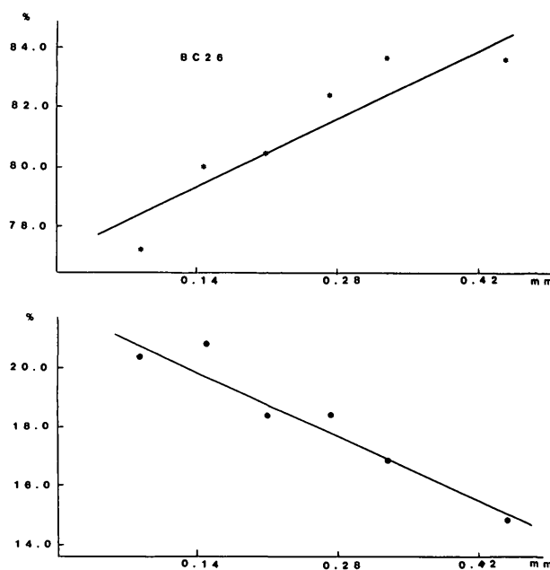
Fig. 3. Total water content (* — *) and nonfreezable water content (as % of the total water) (● — ●), across bovine cornea BC26 as a function of distance (in mm) from the epithelium.
